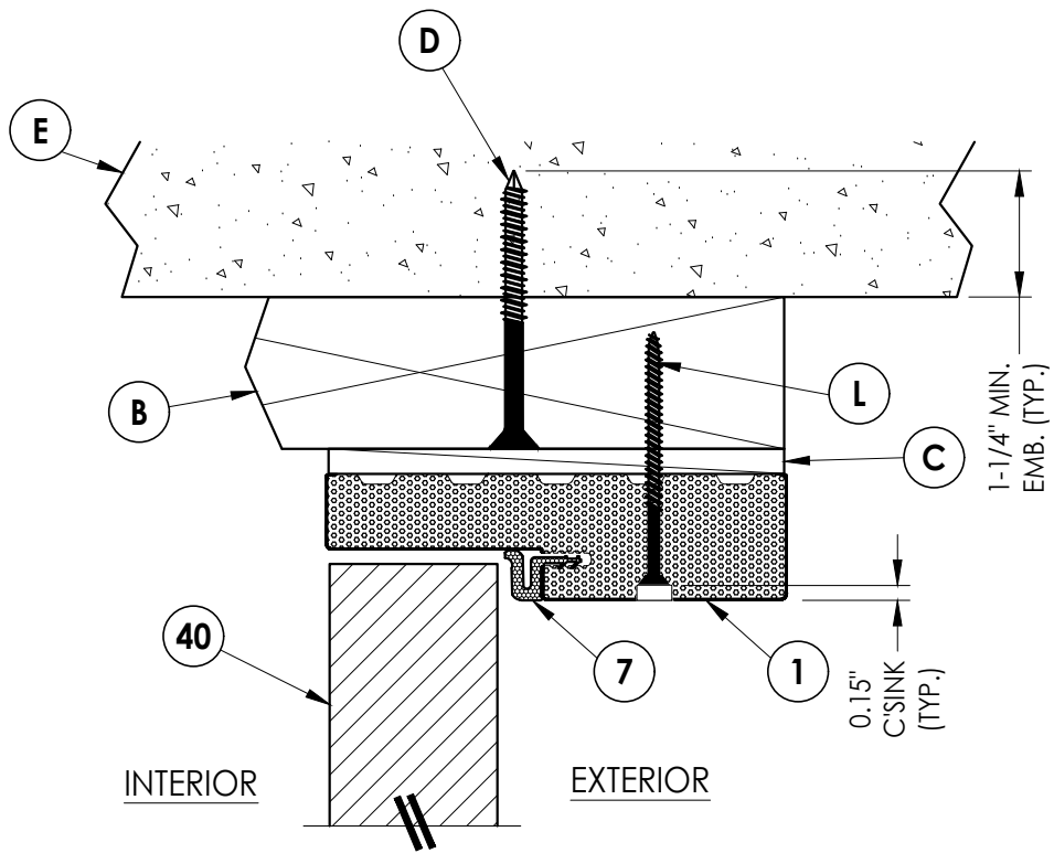
1 4 VERTICAL CROSS SECTION Shown with 2X Buck Inswing
