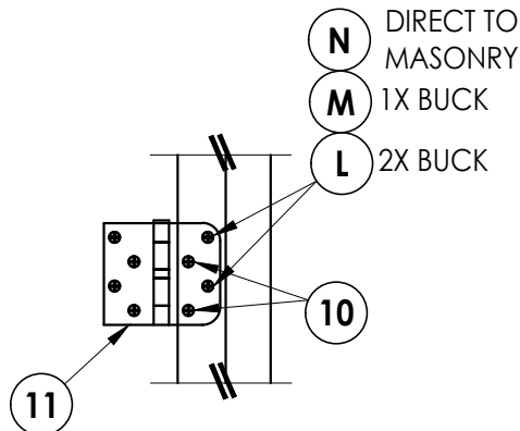
HINGE DETAIL 1
