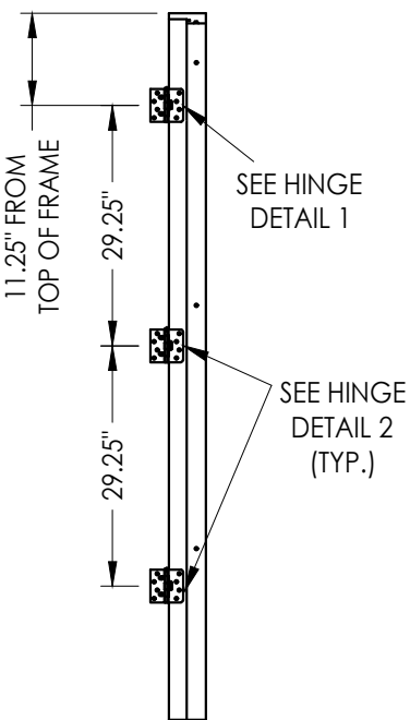
6'8 HINGE JAMB/MULLION
