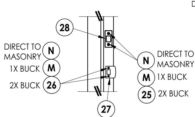
LATCH & DEADBOLT DETAIL
