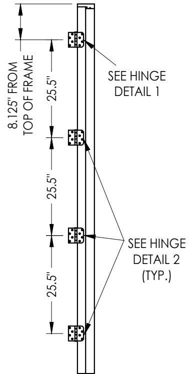
8'0 HINGE JAMB/MULLION
