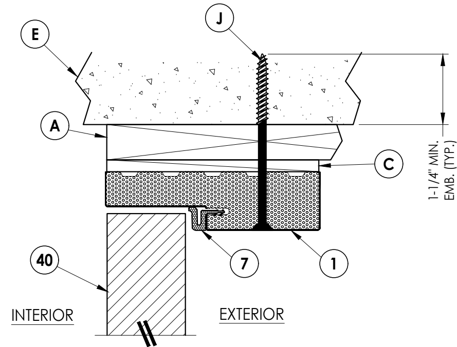
2 4 VERTICAL CROSS SECTION Shown with 1X Buck Inswing
