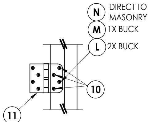
HINGE DETAIL 2
