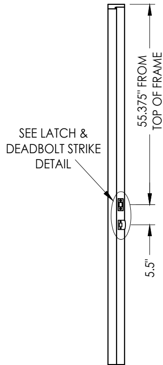
8'0 STRIKE JAMB/MULLION
