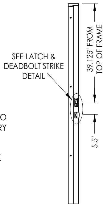
6'8 STRIKE JAMB/MULLION
