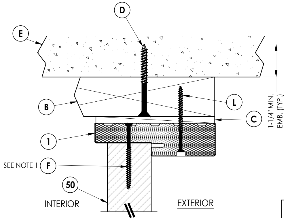
3 4 VERTICAL CROSS SECTION Shown with 2X Buck Inswing
